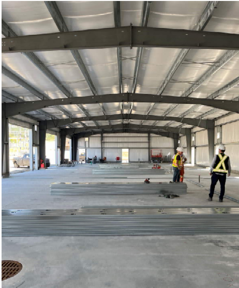
Workshop interior showing completed slab and ongoing steel wall tracks
