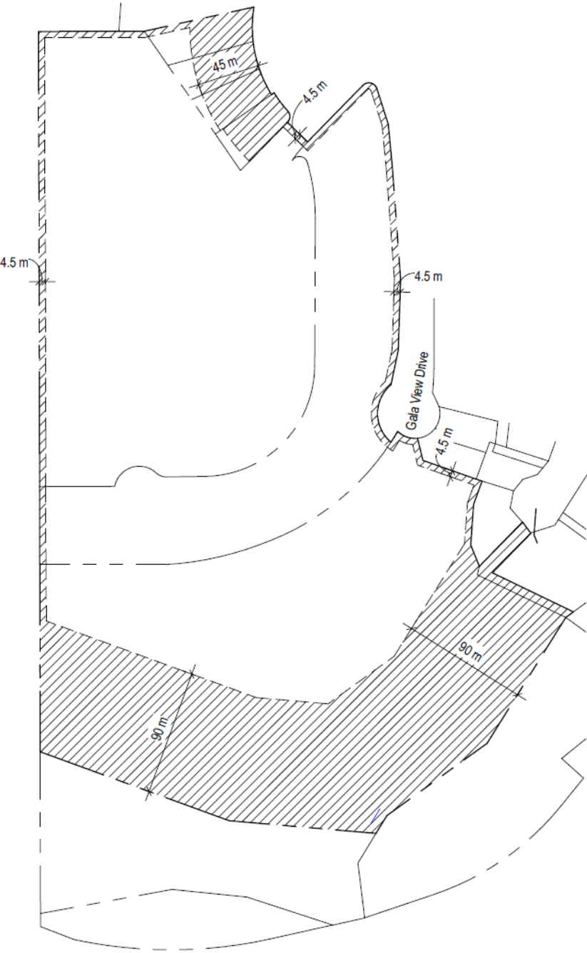
FIGURE 4 - BUILDING SETBACKS
