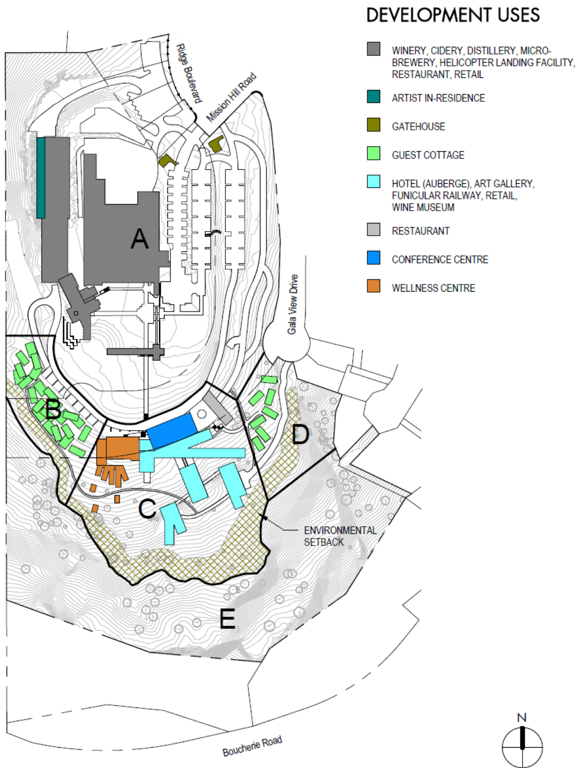
FIGURE 3 - SITE PLAN
