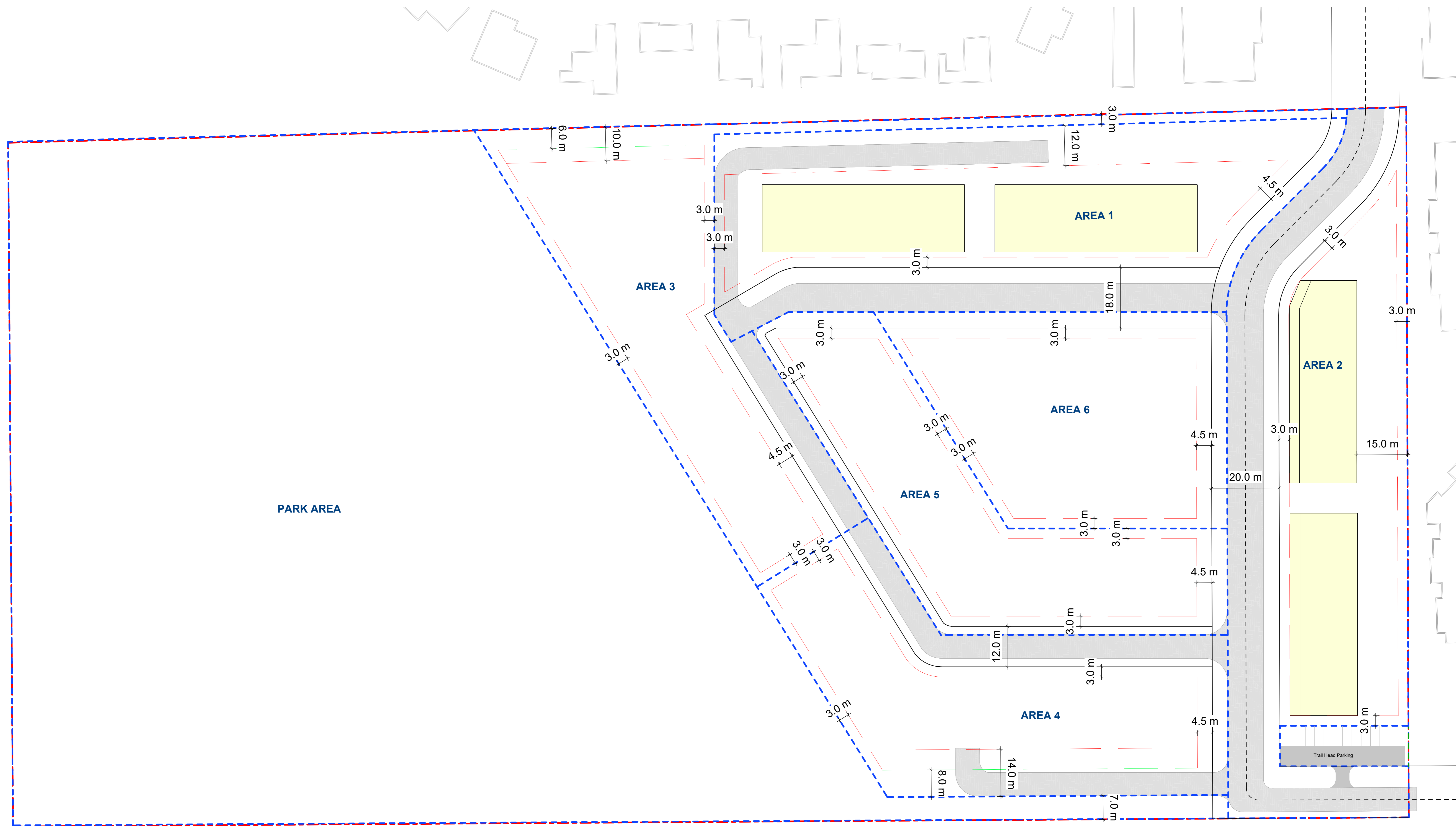
FIGURE 1 - SITE PLAN
