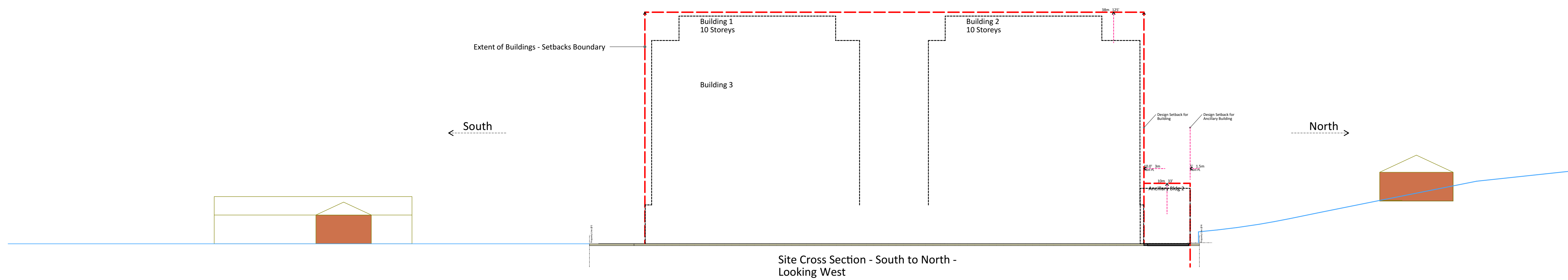
Site Cross Section - South to North
